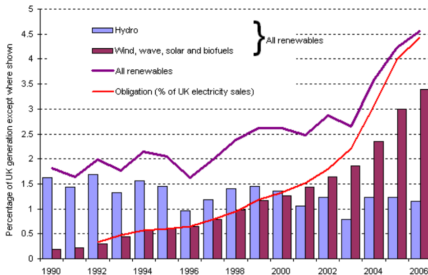
Figure 1.5 - Growth in electricity generation from renewable sources since 1990 (from 'The Digest of United Kingdom Energy Statistics, 2007', BERR).
