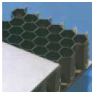
Figure 2.8 - Honeycomb seal for gas turbine engine (Courtesy of Sulzer Metco Turbine Components: Neomet Ltd.).
