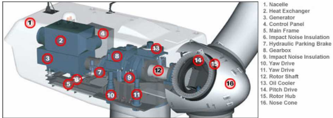
Figure 4.7 - Major components of a wind turbine (from the Scottish Enterprise document: 'Doing Business with the Wind Turbine Manufacturers: Becoming Part of Their Supply Chain', July 2006). (Courtesy of Scottish Enterprise: http://www.scottish-enterprise.com/ ).
