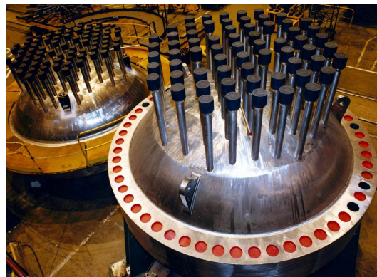
Figure 3.13 – A reactor pressure vessel head showing Control Rod Drive Mechanisms (CRDMs) (Courtesy of Areva: René Quatrain).
