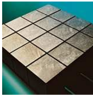
Figure 6.4 – Pure multi-crystalline Si ingot, cut into 'bricks'. (Courtesy of PV Crystalox Solar plc: http://www.crystalox.com/ ).
