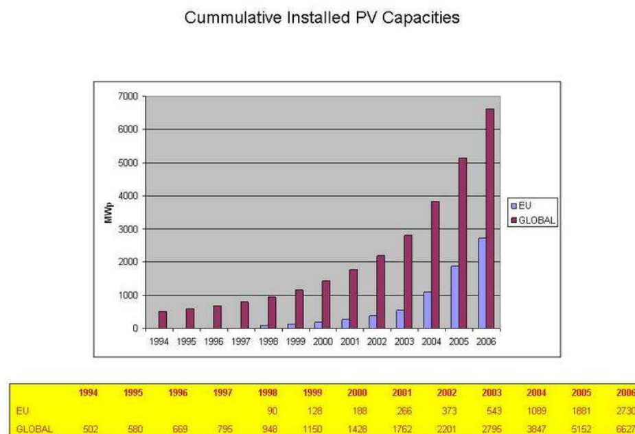
Figure 6.1 - Cumulative global and European installed solar PV capacities. (Courtesy of the European Photovoltaic Industry Association (EPIA): http://www.epia.org/ ).
