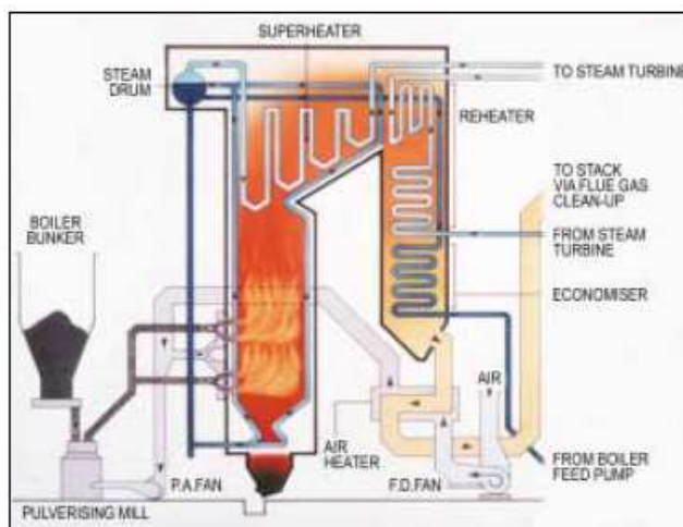
Figure 2.2 - Schematic of a pulverised fuel boiler (from: 'UK Capability: Pulverised Coal-Fired Power Station Boilers', DTI Capability Brochure CB010, March 2001 (DTI/Pub URN 01/593)).
