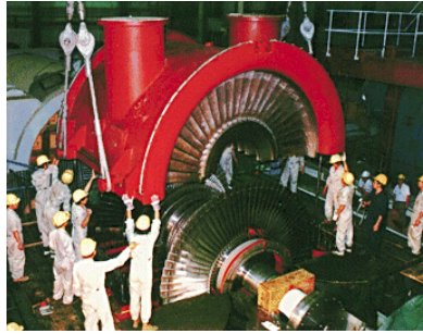
Figure 2.5 – A turbine casing being lowered into position, showing rotor blades fixed blades (nozzles, vanes or diaphragms).
