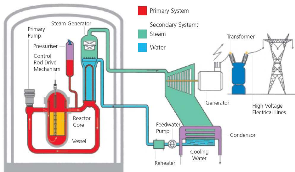
Figure 3.8 – Operational diagram of a typical PWR (from ‘The UK Capability to Deliver a New Nuclear Build Programme’, the NIA, March 2006. (Courtesy of the NIA: http://www.niauk.org/ ).
