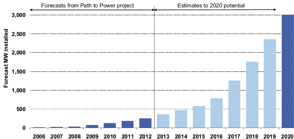
Figure 5.2 - Deployment scenario for wave and tidal energy in the UK to 2020 (from: 'The Path to Power', available at the British Wind Energy Association (BWEA) website: www.bwea.com/pathtopower ). (Courtesy of BWEA).
