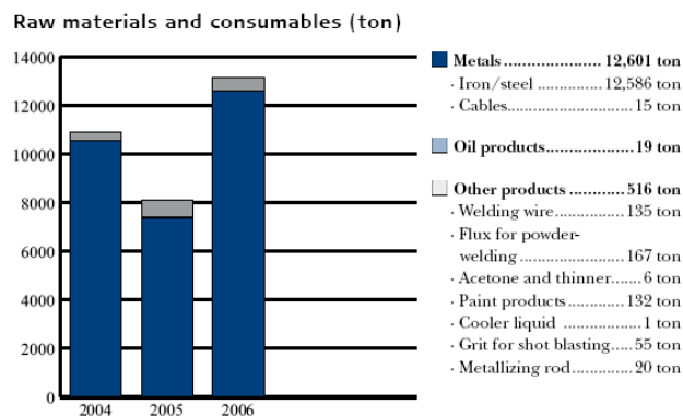
Figure 4.15 - Raw materials and consumables used at the Vestas Campbeltown site. From: 'Environmental Statement 2006 - Company Site. Vestas Towers and Nacelles, Campbeltown, Scotland'. (Courtesy of Vestas: http://www.vestas.com ).
