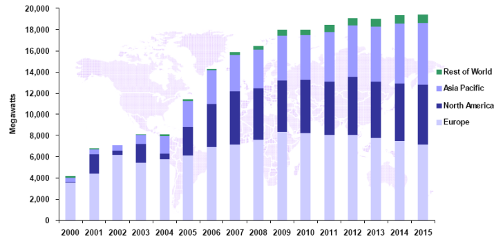
Figure 4.1 - Global wind power capacity increase by year. (Courtesy of Emerging Energy Research: http://www.emerging-energy.com/emerging_markets.html ).
