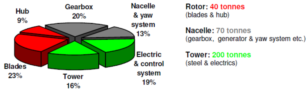
Figure 4.8 – Approximate weights and costs of wind turbine components. (Courtesy of BVG Associates Ltd.).
