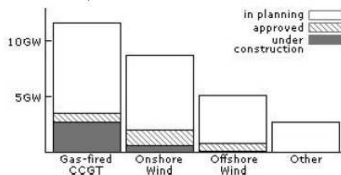
Figure 2.1 - Short-term proposed new electricity generation (from The Parliamentary Office of Science and Technology 'Postnote', February 2007, Number 280).
