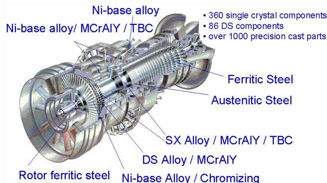
Figure 2.6 – Schematic of a gas turbine engine annotated with some of the materials of construction. (Courtesy of Alstom Power Ltd.).
