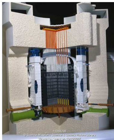
Figure 3.4 - Schematic of the Heysham II / Torness AGR, commissioned in 1988. (Courtesy of 'The Science & Society Picture Library': http://www.scienceandsociety.co.uk/ )
