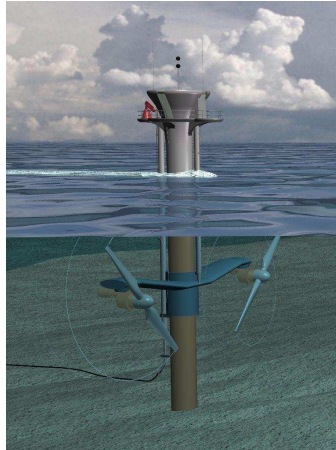
Figure 5.6 – Artist's impression of Marine Current Turbine's 'SeaGen' tidal current turbine. (Courtesy of Marine Current Turbines Ltd: http://www.marineturbines.com/ ).
