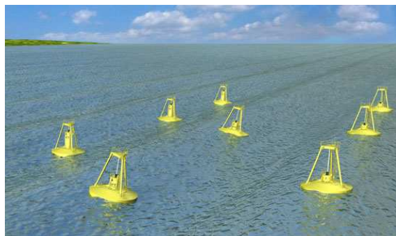
Figure 5.12 – An artist's impression of an array of Ocean Power Technologies PowerBuoy® devices. (Courtesy of Ocean Power Technologies Ltd.: ( http://www.oceanpowertechnologies.com )).
