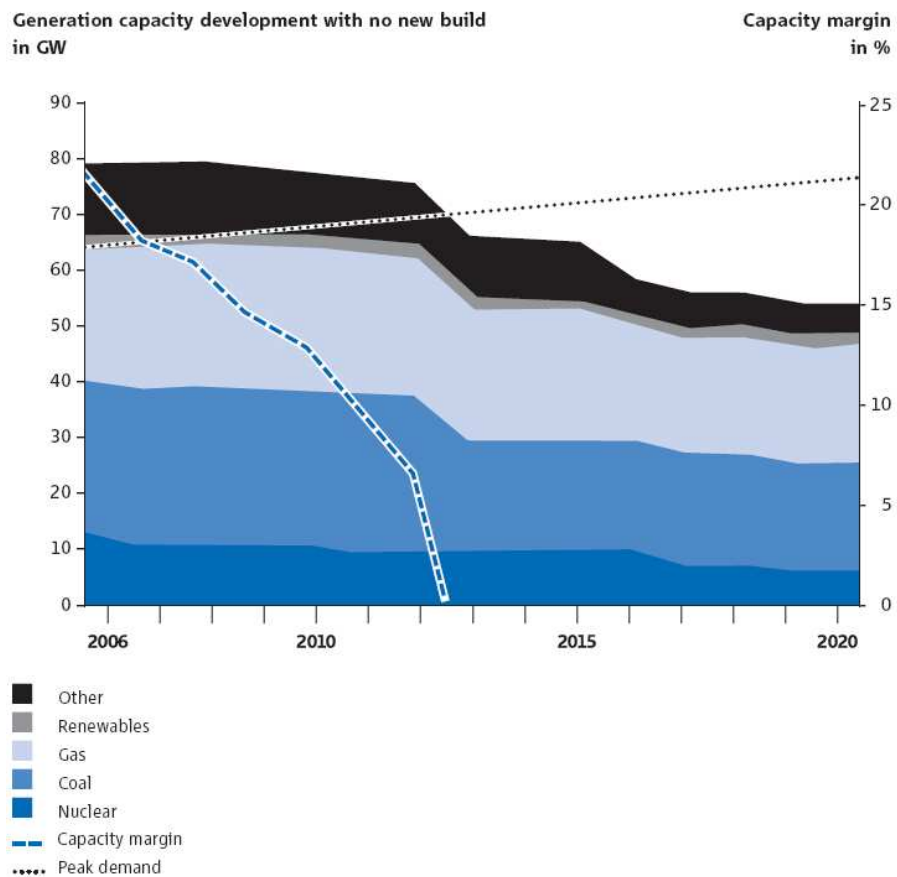
Figure 1.2 - UK electricity generating capacity shut-downs (from RWE 'Facts & Figures 2007', courtesy RWE npower plc: http://www2.rwecom.geber.de/factbook/en/servicepages/welcome ).
