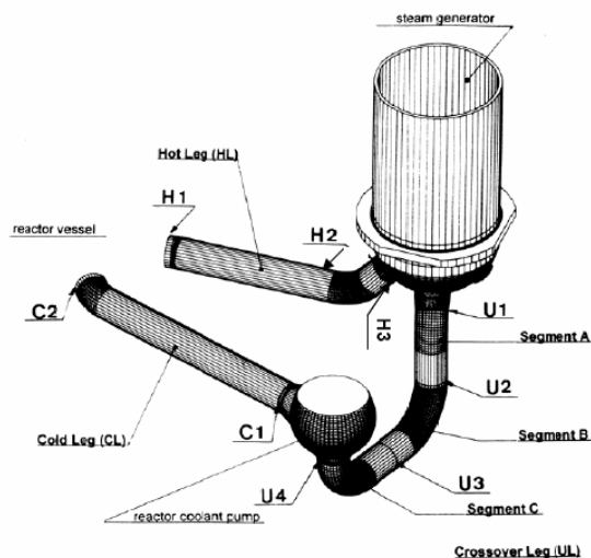
Figure 3.17 - Schematic diagram of Primary Loop (or Circuit) pipework for the Areva NP EPR. (Courtesy of Areva NP: http://www.epr-reactor.co.uk/ ).
