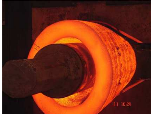
Figure 3.10 - Large Reactor Pressure Vessel (RPV) forging. (Courtesy of Areva NP).
